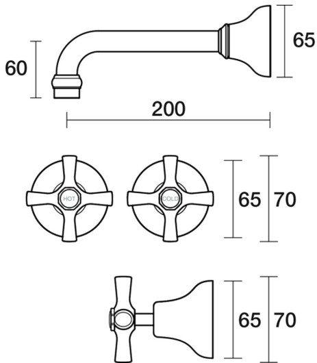
Bell Wall Basin Set 200mm Outlet Ceramic Disc B32.152.2.19 - 23k Brushed Brass Gold
