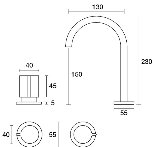
Q Basin Set Swivel B36.011.1.43 - Brass
