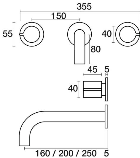
Q Wall Bath Set Outlet 200mm B36.021.1.26 - Black Sapphire
