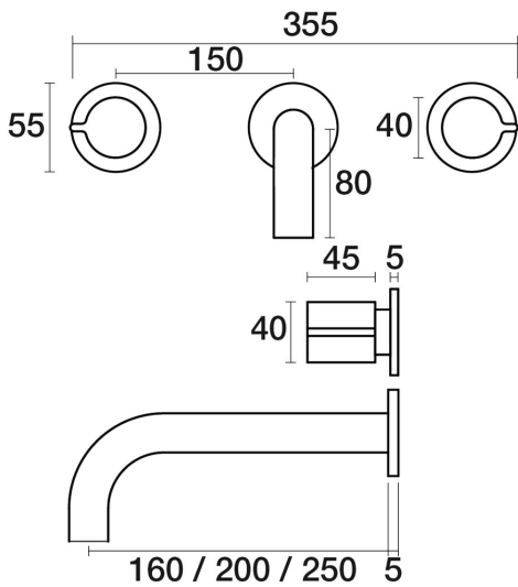
Q Wall Bath Set Outlet 200mm B36.021.1.43 - Brass
