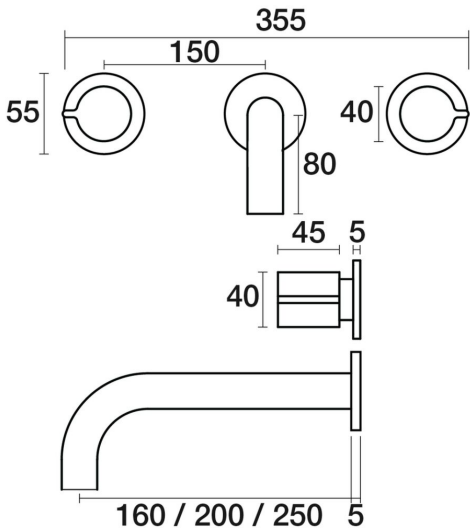
Q Wall Bath Set Outlet 160mm B36.021.2.01 - Chrome
