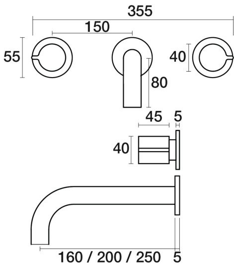
Q Wall Bath Set Outlet 160mm B36.021.2.25 - Brushed Nickel
