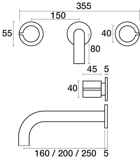
Q Wall Bath Set Outlet 160mm B36.021.2.43 - Brass
