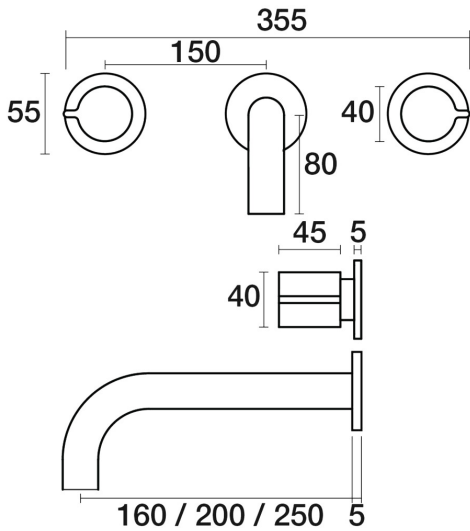
Q Wall Bath Set Outlet 160mm B36.021.2.52 - Burnished
