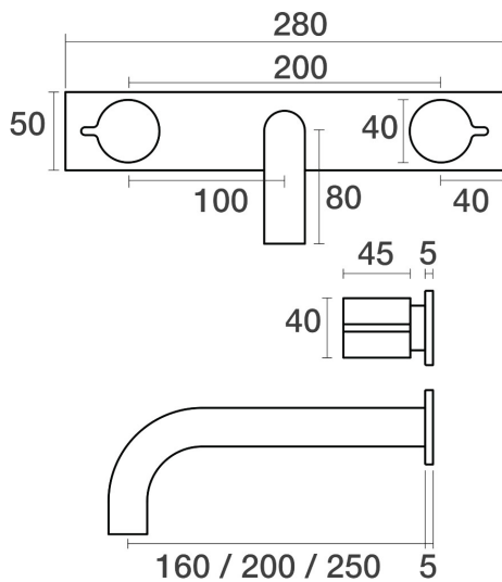
Q Wall Bath Set Outlet 200mm on Plate B36.021.4.44 - Antique Copper
