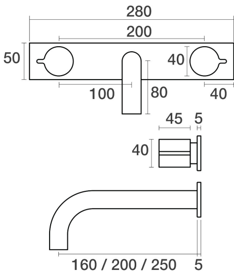
Q Wall Bath Set Outlet 250mm on Plate
