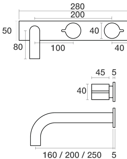
Q Wall Bath Set Outlet 200mm on Plate - Offset B36.021.7.40 - Rumbled Brass
