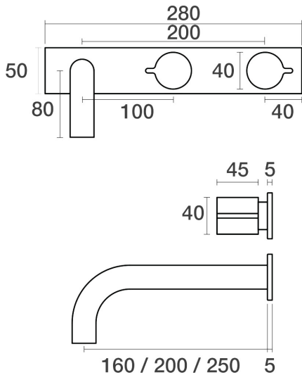
Q Wall Bath Set Outlet 200mm on Plate - Offset B36.021.7.67 - Vintage Brass
