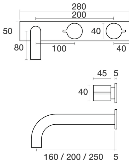
Q Wall Bath Set Outlet 160mm on Plate - Offset B36.021.8.11 - 23k Gold
