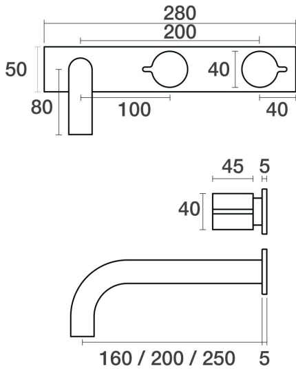
Q Wall Bath Set Outlet 250mm on Plate - Offset B36.021.9.01 - Chrome
