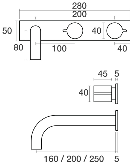
Q Wall Bath Set Outlet 250mm on Plate - Offset B36.021.9.40 - Rumbled Brass
