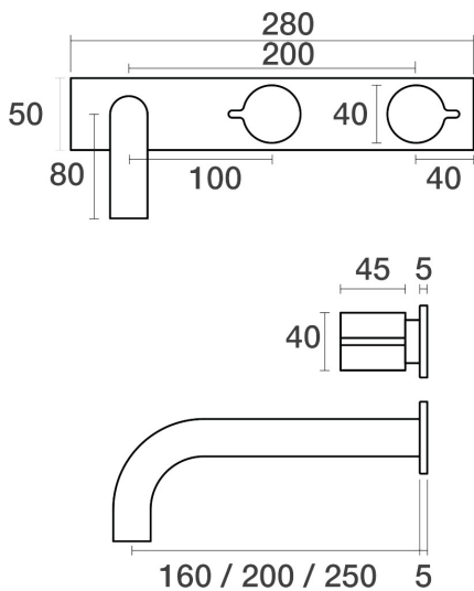
Q Wall Bath Set Outlet 250mm on Plate - Offset B36.021.9.41 - Brushed Brass
