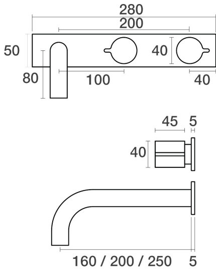
Q Wall Bath Set Outlet 250mm on Plate - Offset B36.021.9.42 - Brushed Copper
