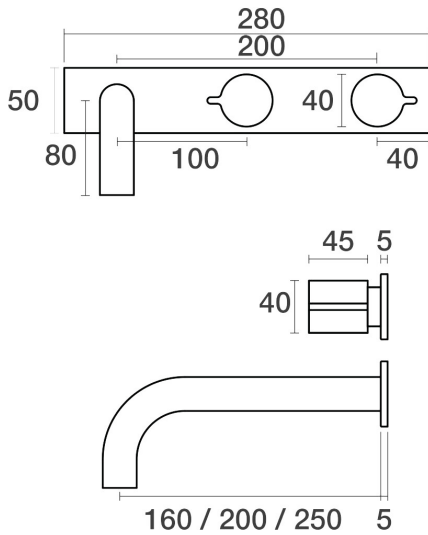
Q Wall Bath Set Outlet 250mm on Plate - Offset B36.021.9.67 - Vintage Brass
