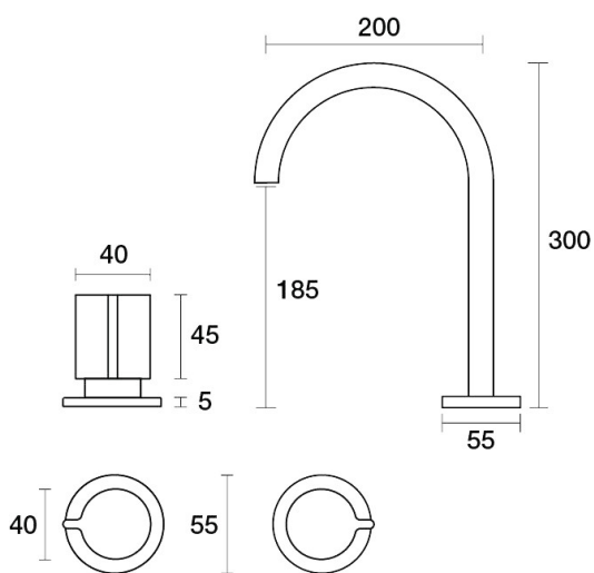
Q Spa Set Hob Swivel B36.061.1.52 - Burnished
