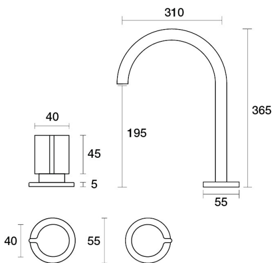
Q Spa Set XL Hob Swivel B36.063.1.48 - Copper
