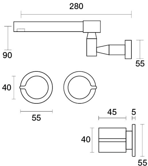
Q Spa Set XL Wall Swivel B36.064.1.27 - Satin Pearl
