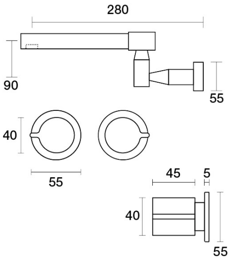
Q Spa Set XL Wall Swivel B36.064.1.32 - Midnight Black
