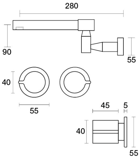
Q Spa Set XL Wall Swivel B36.064.1.45 - Native Brass
