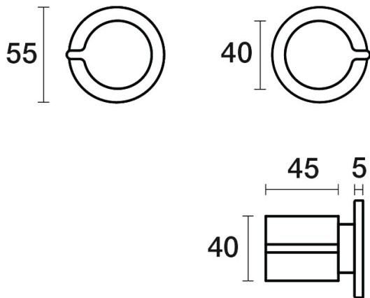
Q Top Assemblies Wall Pair B36.082.1.43 - Brass
