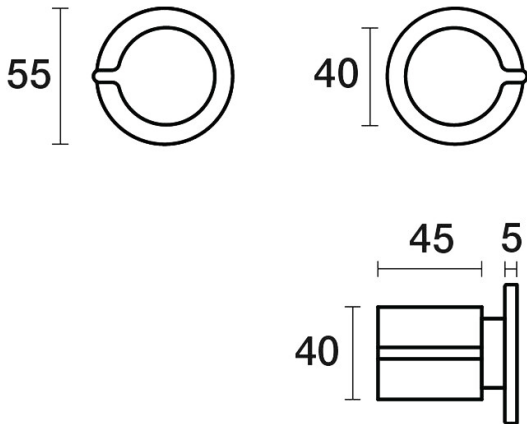
Q Top Assemblies Wall Pair B36.082.1.44 - Antique Copper
