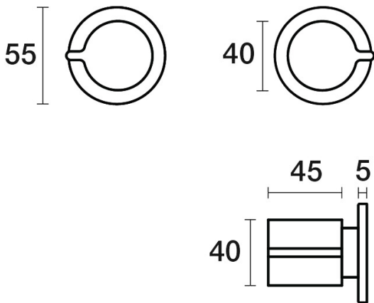
Q Top Assemblies Wall Pair B36.082.1.68 - Autumn Bronze
