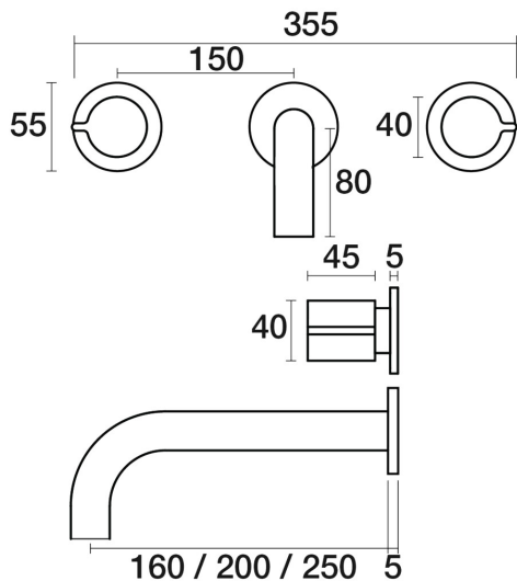
Q Wall Basin Set Fixed Outlet 200mm B36.152.1.27 - Satin Pearl
