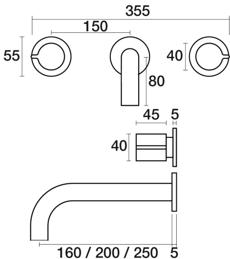
Q Wall Basin Set Fixed Outlet 200mm B36.152.1.47 - Luminick
