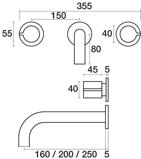
Q Wall Basin Set Fixed Outlet 200mm B36.152.1.48 - Copper
