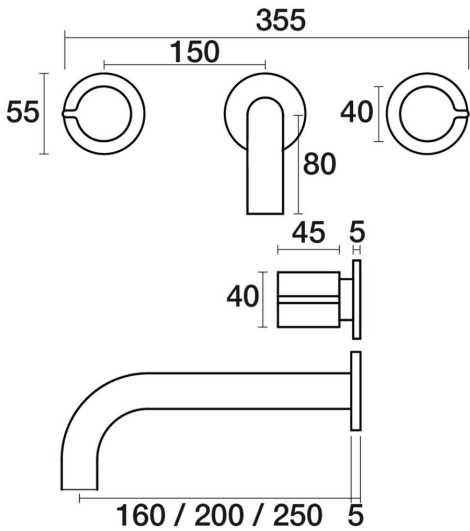
Q Wall Basin Set Fixed Outlet 160mm B36.152.2.01 - Chrome
