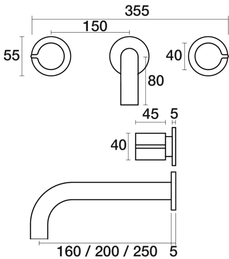
Q Wall Basin Set Fixed Outlet 160mm B36.152.2.40 - Rumbled Brass
