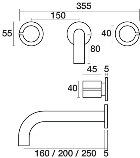
Q Wall Basin Set Fixed Outlet 250mm B36.152.3.01 - Chrome
