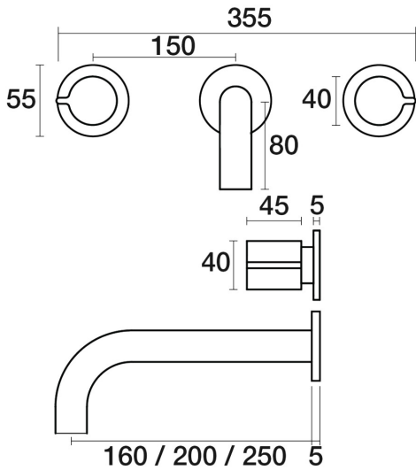
Q Wall Basin Set Fixed Outlet 250mm B36.152.3.34 - Matt Black
