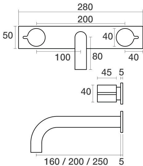
Q Wall Basin Set Fixed Outlet 200mm on Plate B36.152.4.24 - Brushed Gunmetal
