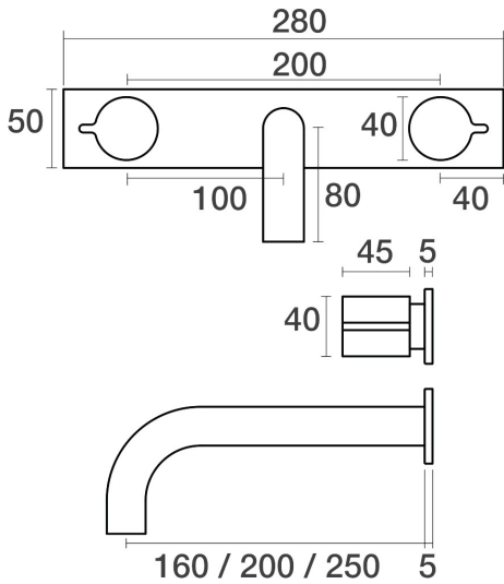
Q Wall Basin Set Fixed Outlet 200mm on Plate B36.152.4.34 - Matt Black
