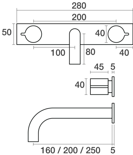
Q Wall Basin Set Fixed Outlet 160mm on Plate B36.152.5.01 - Chrome
