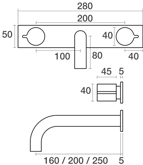
Q Wall Basin Set Fixed Outlet 250mm on Plate B36.152.6.32 - Midnight Black
