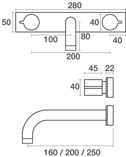
QWC Wall Bath Set Outlet 250mm on Plate B37.021.6.01 - Chrome
