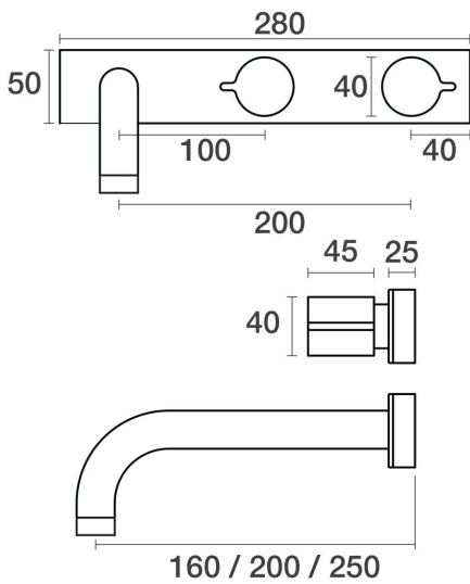
QWC Wall Basin Set Fixed Outlet 200mm on Plate - Offset
