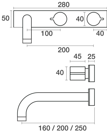
QWC Wall Basin Set Fixed Outlet 160mm on Plate - Offset
