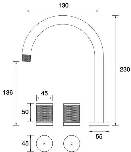
IDK Basin Set Swivel B38.011.2.01 - Chrome
