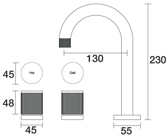
IDK Basin Set Swivel B38.011.2.01 - Chrome
