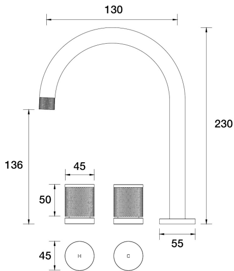
IDK Basin Set Swivel B38.011.2.27 - Satin Pearl
