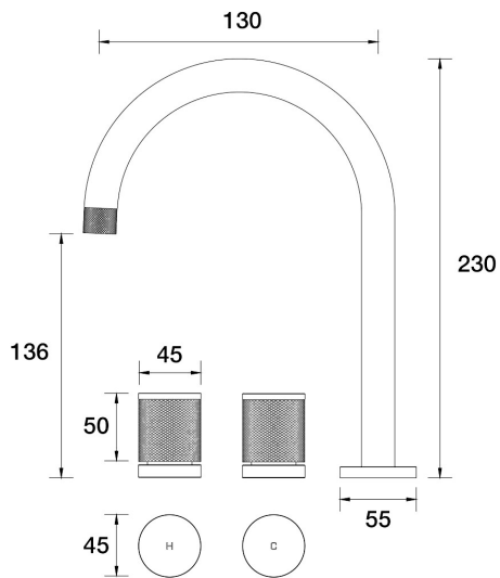
IDK Basin Set Swivel B38.011.2.44 - Antique Copper
