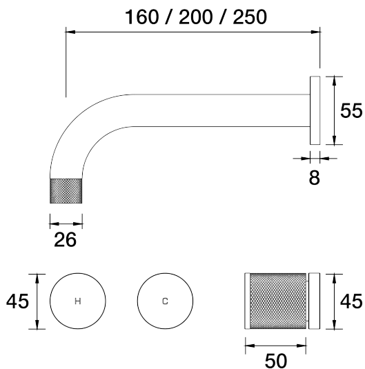
IDK Wall Bath Set 160mm Outlet B38.021.2.01 - Chrome
