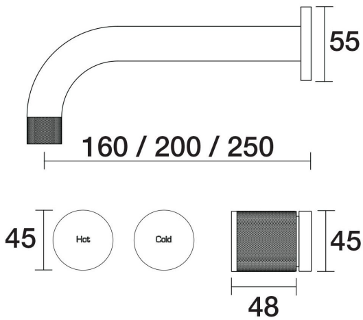
IDK Wall Bath Set 160mm Outlet B38.021.2.01 - Chrome
