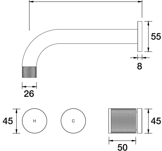
IDK Wall Bath Set 160mm Outlet B38.021.2.39 - Antique Bronze
