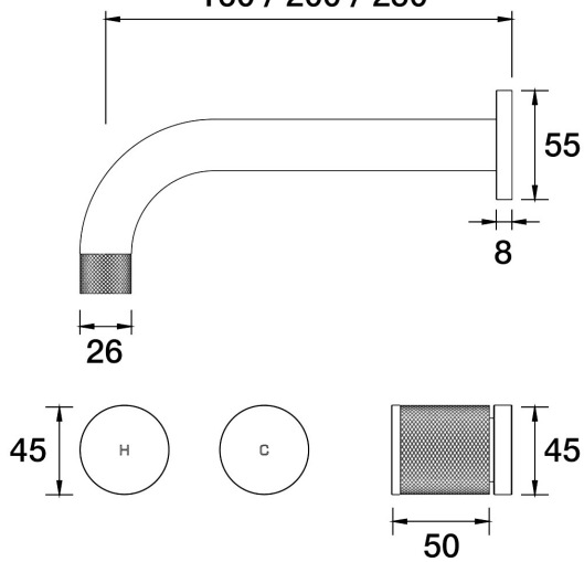
IDK Wall Bath Set 160mm Outlet B38.021.2.52 - Burnished
