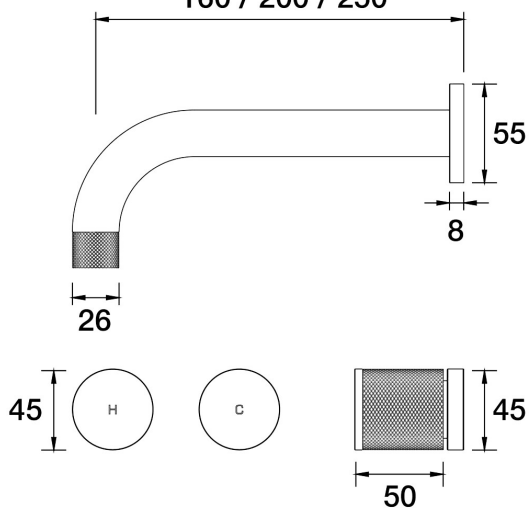
IDK Wall Bath Set 160mm Outlet B38.021.2.78 - Umber Earth
