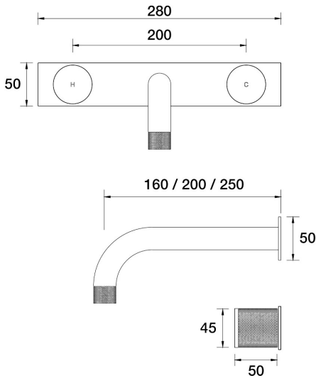
IDK Wall Bath Set 160mm Outlet on Plate B38.021.4.27 - Satin Pearl
